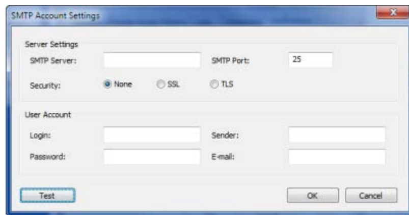
Fig. 76 – SMTP settings
