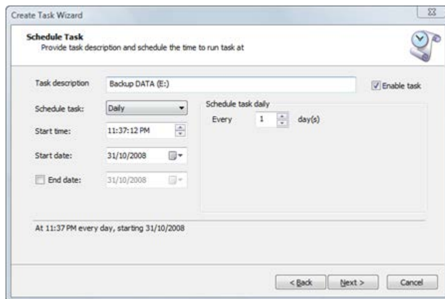
Fig. 61 – Schedule Task
